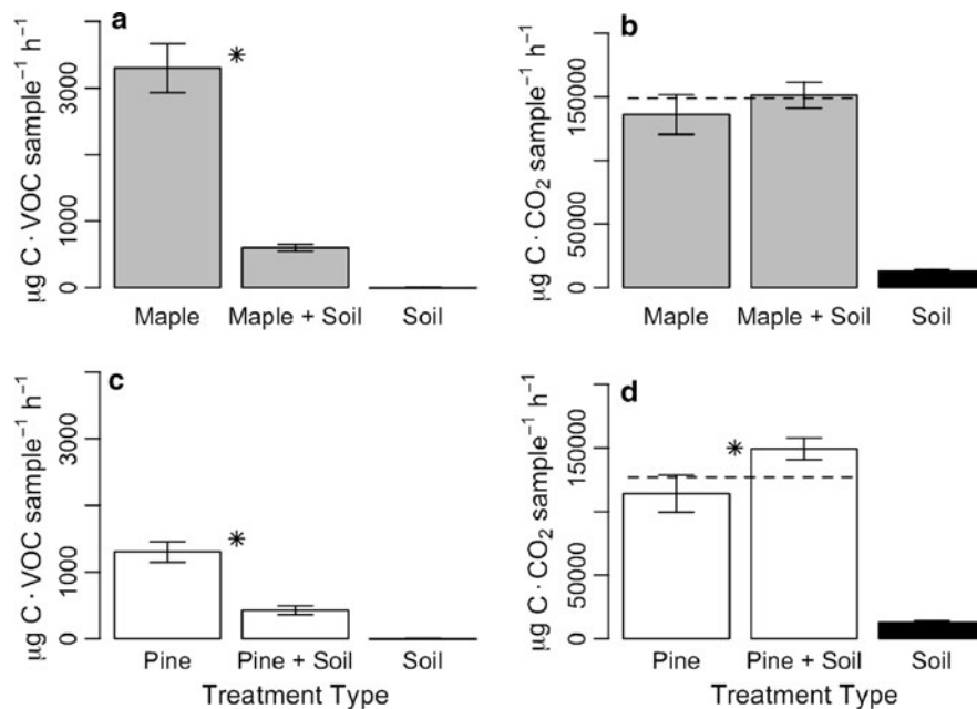
Fig. 5 Total VOC and CO 2 emissions for each treatment type. a Total VOC Production for maple treatments. b Total CO 2 production for maple treatments. c Total VOC production for pine litter plus soil treatments. d Total CO 2 production for pine litter plus soil treatments. Error bars indicate \pm standard error of the mean ( n = 4 ). Hatched lines represent the amount of CO 2 that should be observed if soil and litter emissions were additive. Significant differences between litter alone versus litter plus soil treatments ( p < 0.05 ) are designated with asterisks
